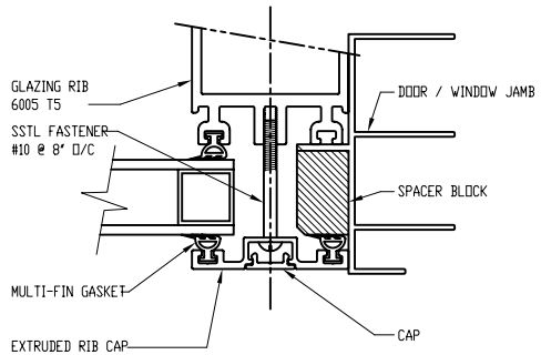
10 SLIDING DOOR / WINDOW JAMB SCALE: NONE
