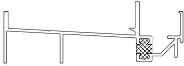
MAIN SILL
