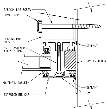
3 GLAZING RIB AT JAMB SCALE: NONE
