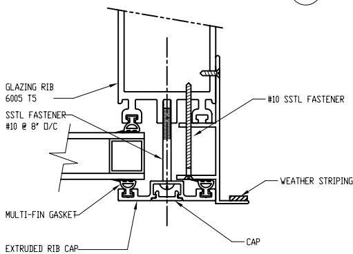
10 SLIDING DOOR / WINDOW JAMB SCALE: NONE
